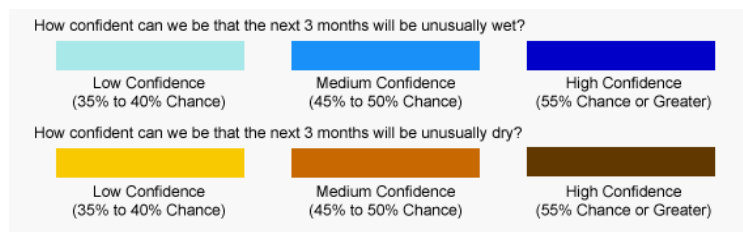
Forecast for Sep-Nov 2011, Forecast Issued Aug 2011
