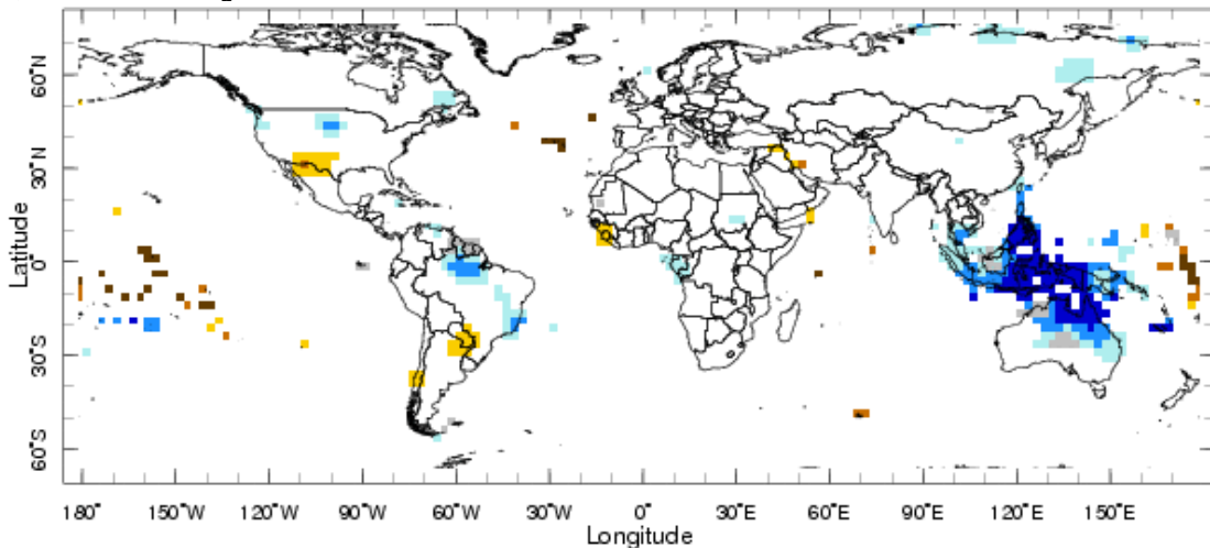
Forecast for Sep-Nov 2011, Forecast Issued Aug 2011
