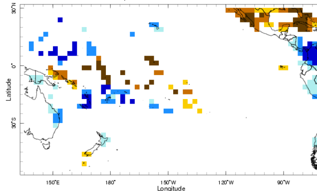
Forecast for Dec 2010 - Feb 2011, Forecast Issued Nov 2010
