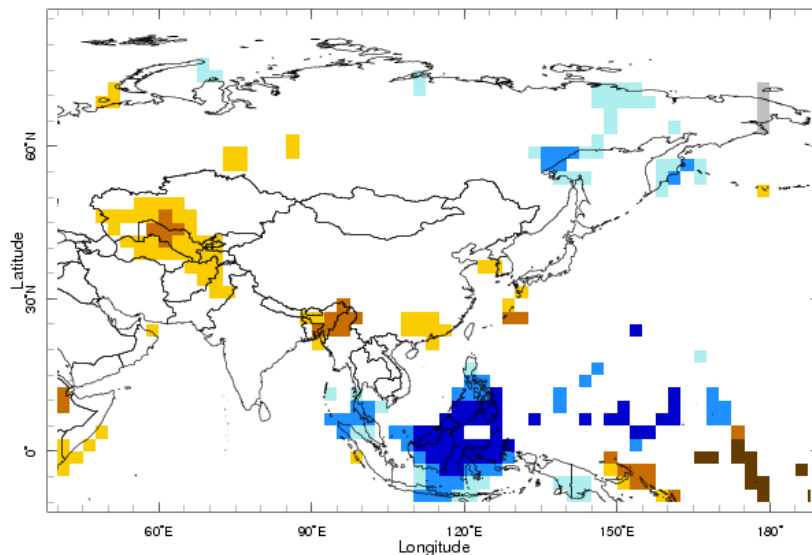
Forecast for Dec 2010 - Feb 2011, Forecast Issued Nov 2010
